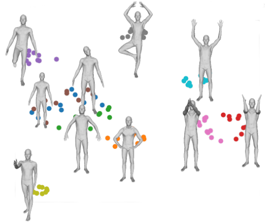
Figure 1: 2D visualization of the FAUST dataset by our method using t-SNE algorithm based on the metric from equation 5. The metric parameters are set to a = 1, \lambda = 0.0001, c = 0 . Each color represents a class of pose and a class representative is also displayed.
