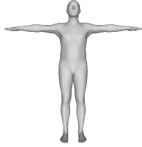
Figure 6: SMPL template
