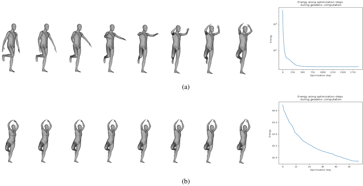
Figure 3: Examples of geodesic path between f_1 and far left and f_2 far right: (a) with metric parameters ( a=1, \lambda = 1, c=0 ), (b) with metric parameters ( a=0, \lambda = 0, c=1 ). The corresponding energy evolution during optimization are displayed on the right. Computation time was respectively 3min31s and 10.6s.
