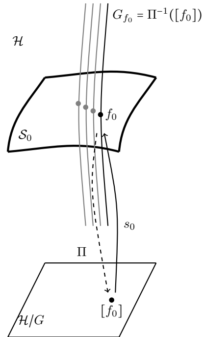
Figure 9: Section of the fiber bundle \Pi : \mathcal{H} \rightarrow \mathcal{H}/G : the one-to-one correspondence with the template mesh allows us to work on the corresponding section \mathcal{S}_0 as a shape space. The correspondance initially gives the section for \text{Diff}^+(\mathcal{T}) , but with Procrustes analysis, the section for \text{SO}(3) comes straightforwardly.
