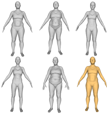
Figure 4: Karcher mean (yellow) for a five different people relatively to the distance with metric parameters ( a = 0, \lambda = 0, c = 1 ).
