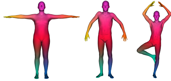
Figure 8: Alignment with the template: The 3 meshes in different poses are displayed with different color on extremities. This validate the choice to work on this particular section of the fiber bundle \Pi : \mathcal{H} \rightarrow \mathcal{H}/G
